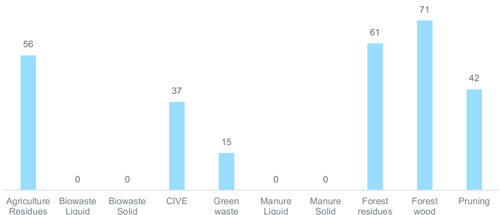
Figure 18: Average cost for feedstock in 2050, €2019/tons
